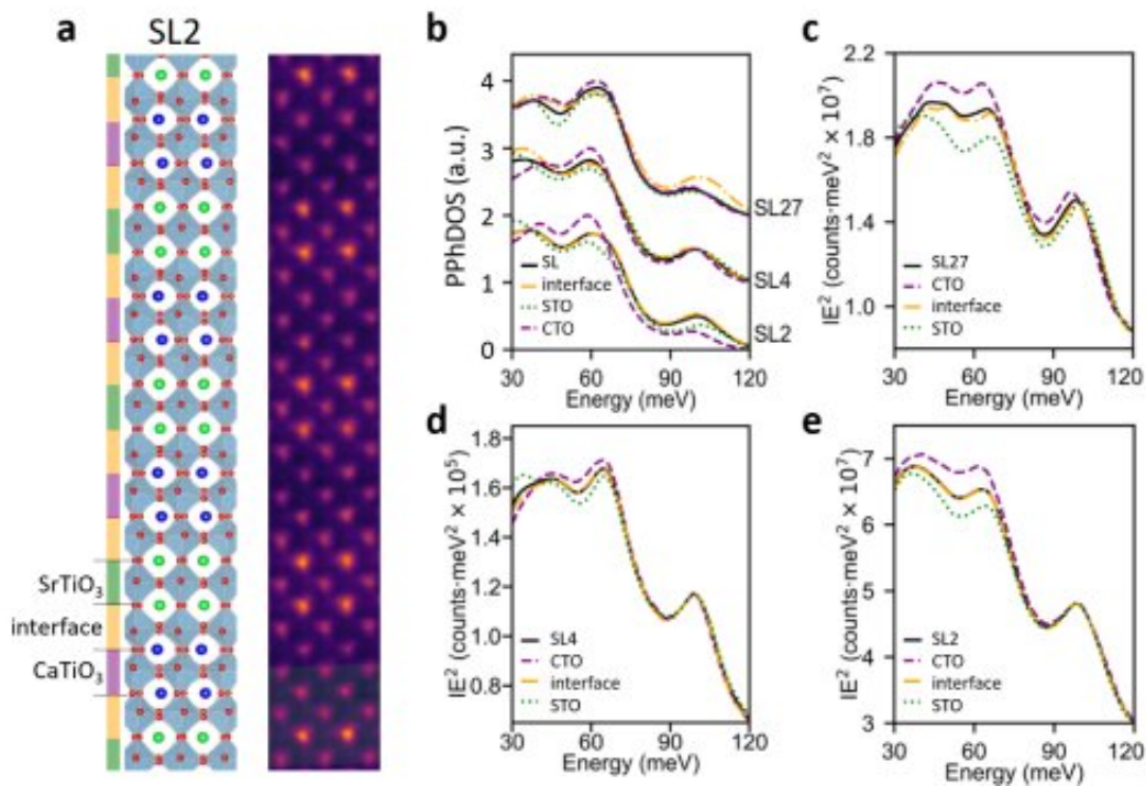
Left: Schematic of the atomic positions in a 2×2 superlattice (SL2); right: atomic-resolution STEM image. Credit: Vanderbilt University
