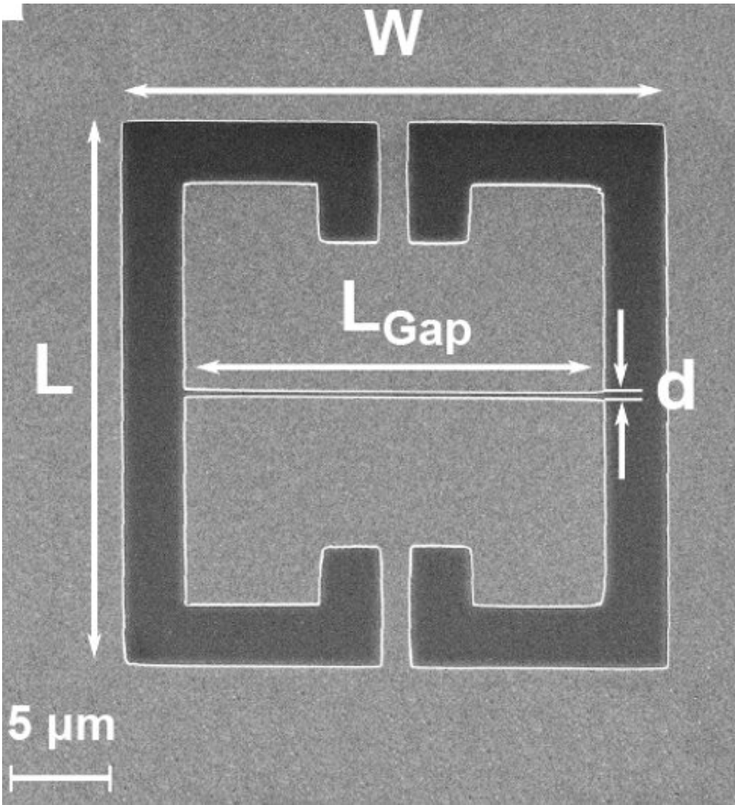
Scanning electron microscope (SEM) image of a unit cell containing a split-ring resonator with a gap of d = 250 nm. Credit: Adapted from S. Rajabali et al. doi: 10.1038/s41566-021-00854-3, Nature Photonics (2021)
