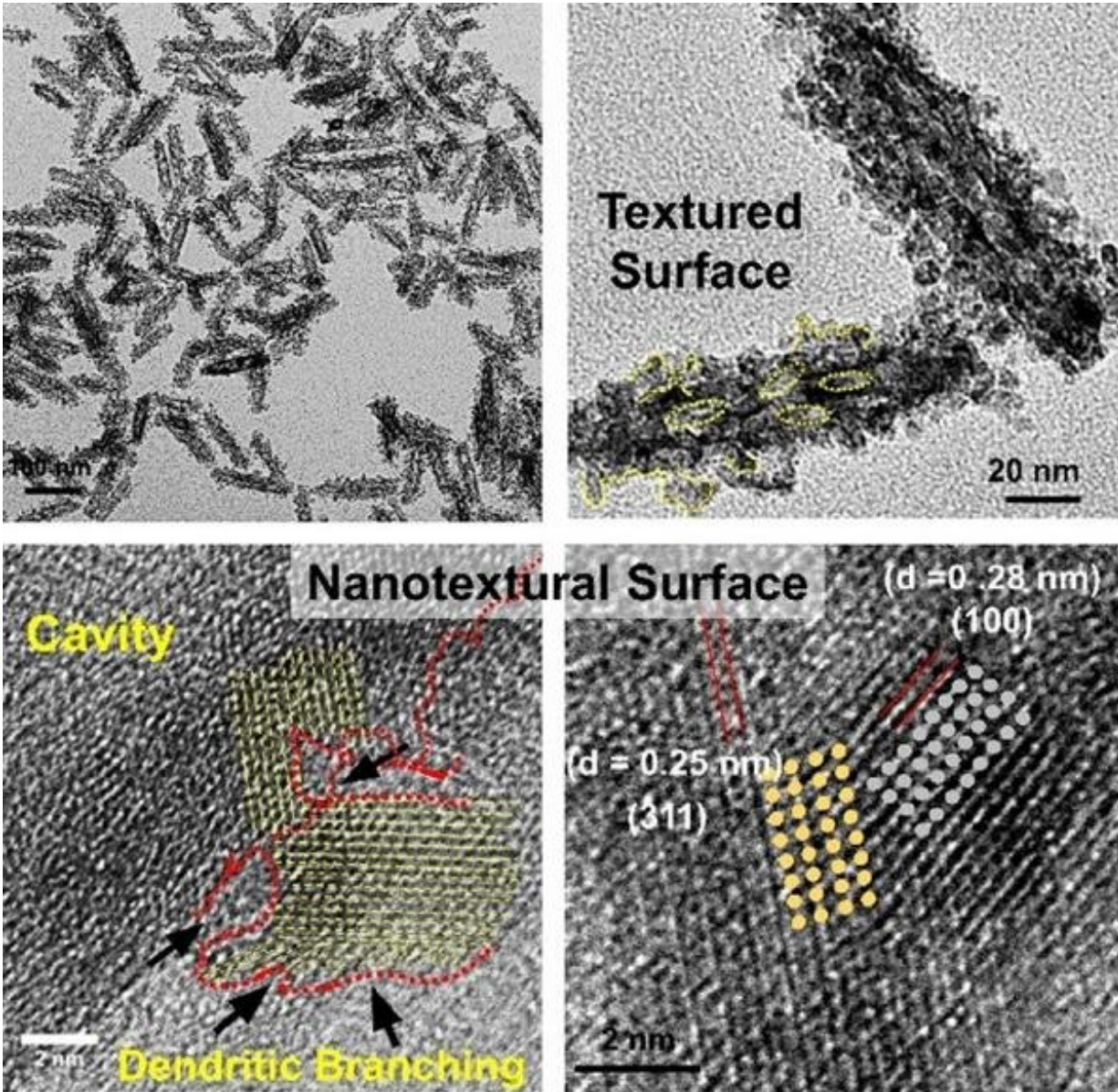
Transmission electron microscope (TEM) image of Mtex
