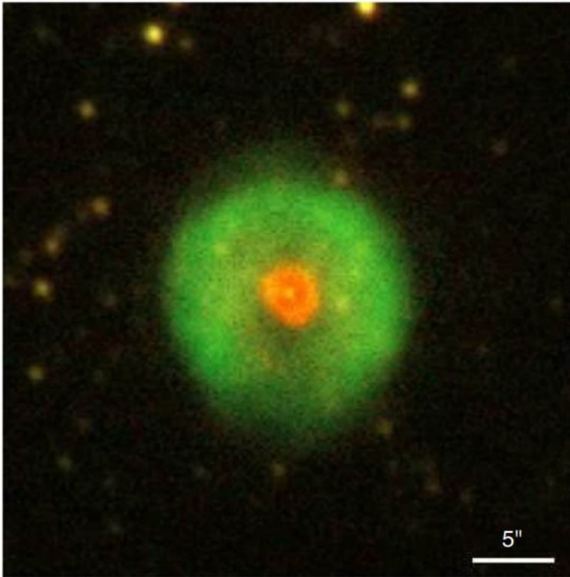
NOT ALFOSC [N ii] \lambda 6584 (red) and H \alpha \lambda 6563 (green) colour composite
