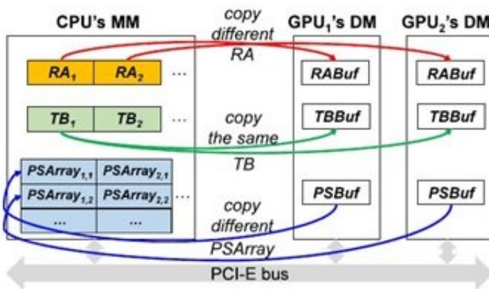
Fig 2. Data flow of GMiner using multiple GPUs. Credit: Daegu Gyeongbuk
