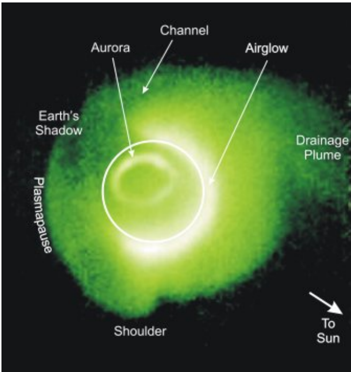
Earth's plasmasphere and plume as measured by IMAGE's Extreme Ultraviolet Imager. Credit: Sandel, B. R., et al., Space Sci. Rev. , 109, 25, 2003
