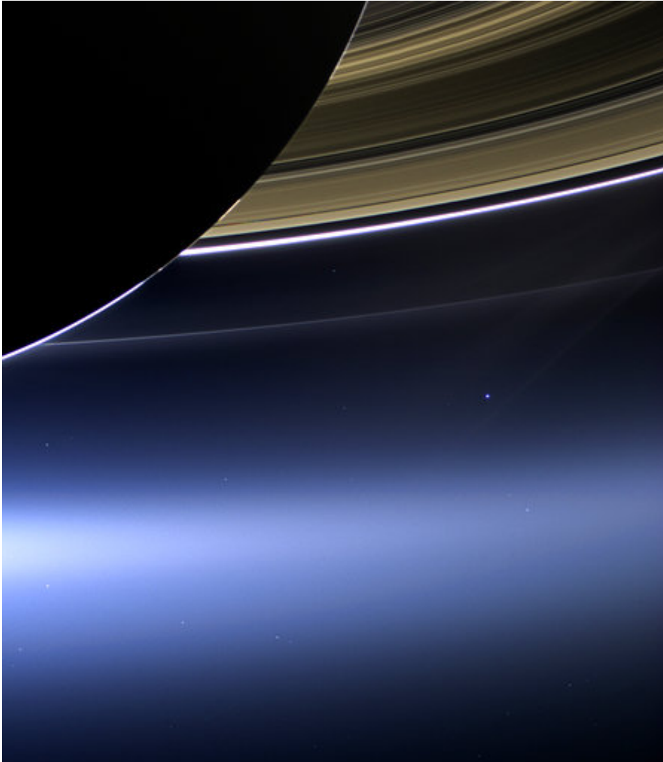
This July 19, 2013 image made available by NASA shows Saturn's rings and planet Earth, center right, as seen from the Cassini spacecraft. (NASA/JPL-Caltech/Space Science Institute via AP)
