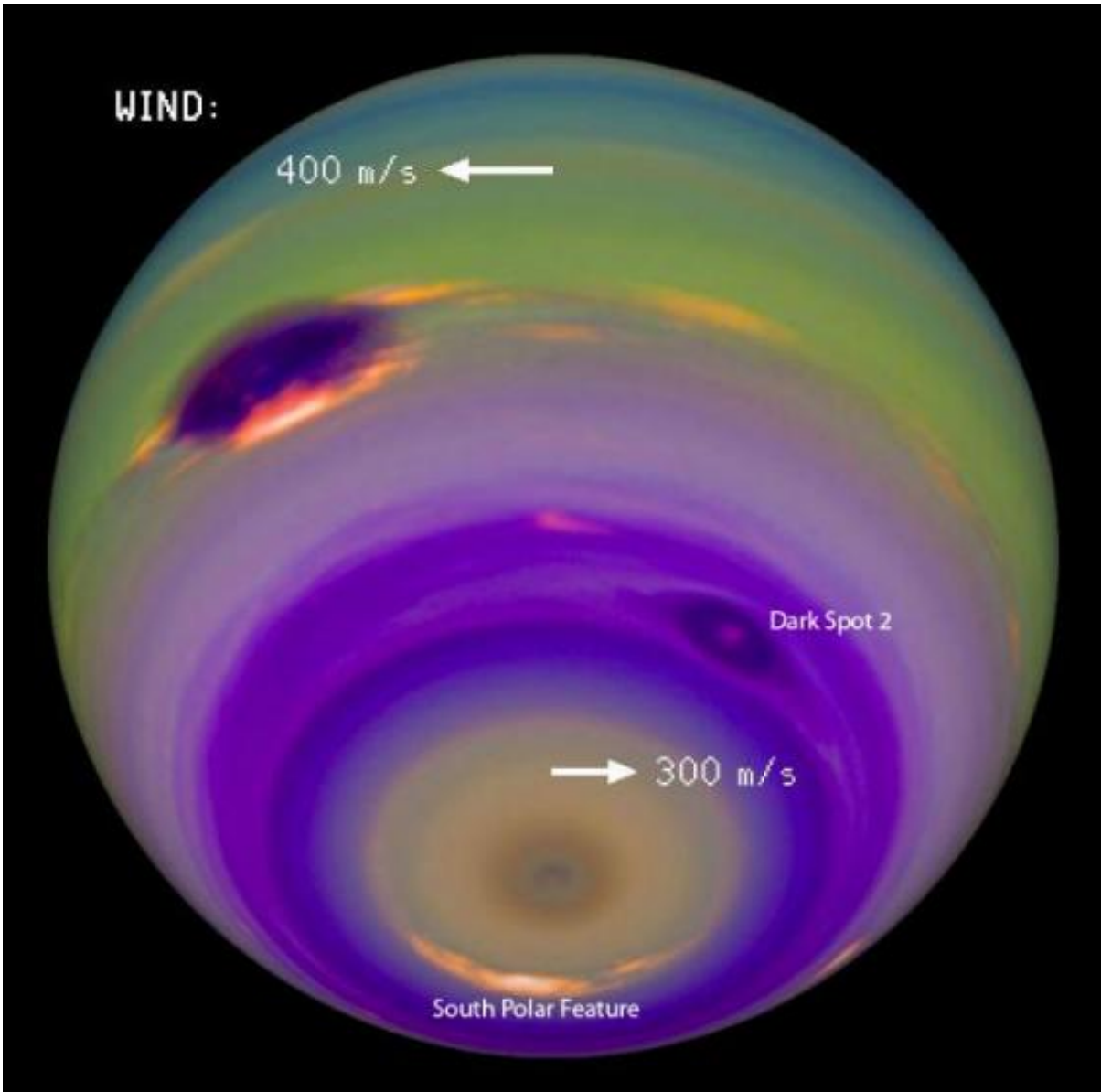
Neptune's atmosphere, with colors contrasts modified to emphasize the planet's atmospheric features. Credit: Erich Karkoschka
