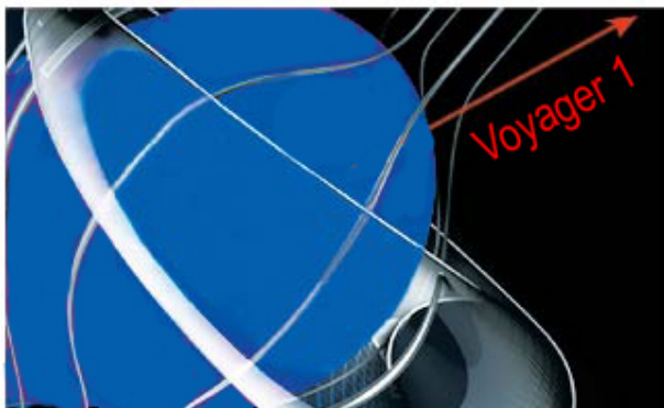
A North-South projection of heliopause and ribbon
