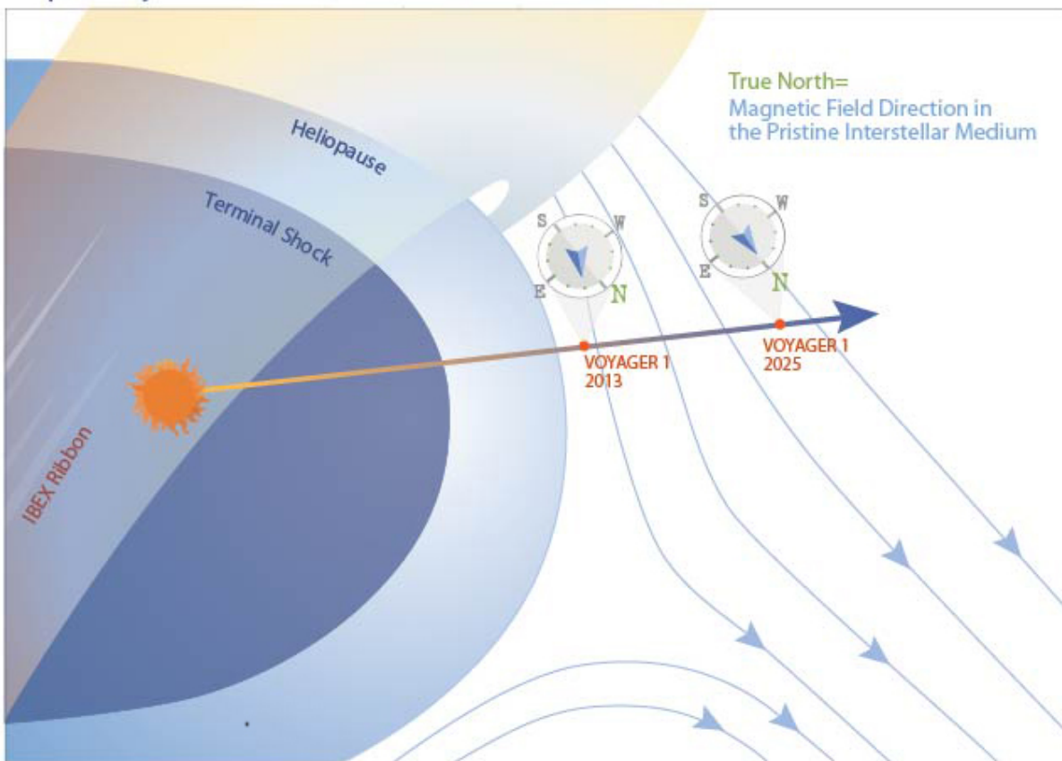
Ecliptic Projection
