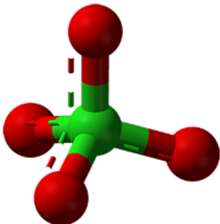
Ball-and-stick model of the perchlorate ion.
