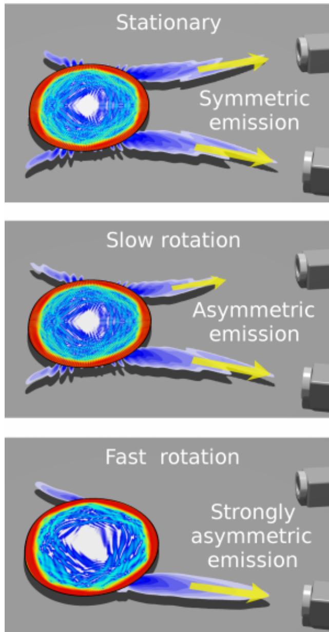
Schematics showing the far-field emission pattern of a microdisk cavity
