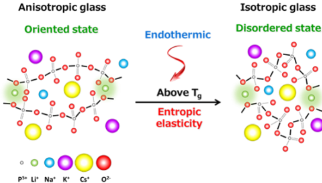
Fig.2: Model of anisotropic glass and isotropic glass.
