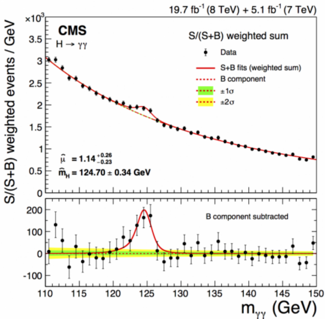
Figure 1: Combined diphoton mass spectrum illustrating the significance of the observed excess, where events are weighted by the expected signal-to-background ratio. The corresponding background-subtracted distribution is shown in the lower panel.
