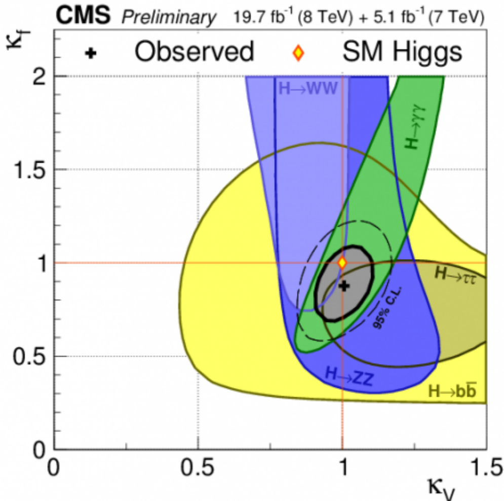
Figure 2: Compatibility of Higgs boson couplings to vector bosons (V) and fermions (f) with the Standard Model expectation (diamond). The allowed regions by each group of decay modes analyzed (coloured) combine into a much smaller region (grey) that is fully compatible with the Standard Model.
