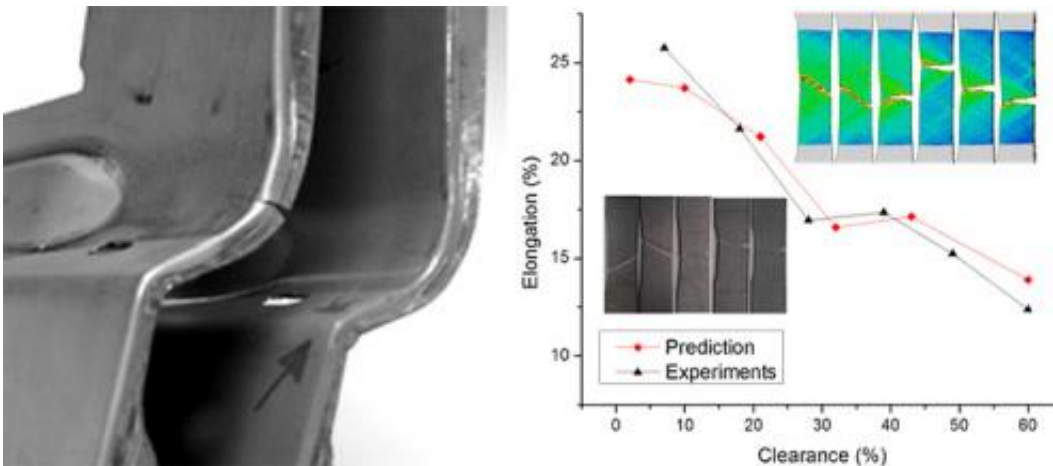
(left) Edge fracture observed in production, and (right) predicted and measured trimmed edge elongation and sample failure modes at different trimming clearances.
