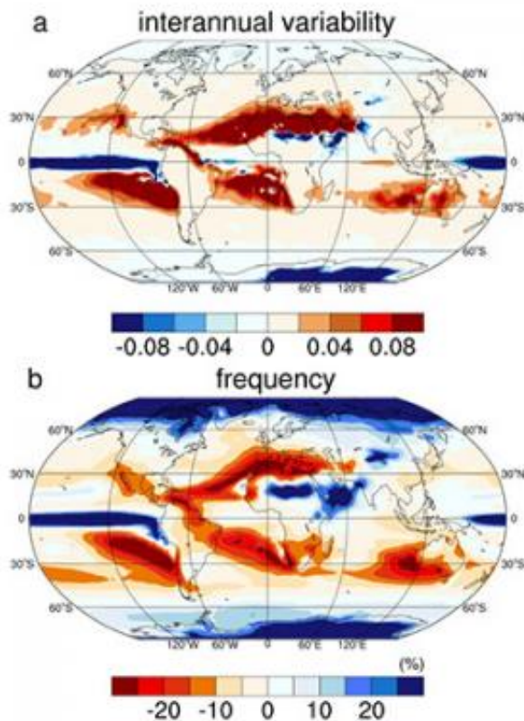
CMIP5 multi-model ensemble average change in (a) interannual variability of precipitation scaled by historical mean annual precipitation; (b) frequency of precipitation days (%). Credit: Scientific Reports
