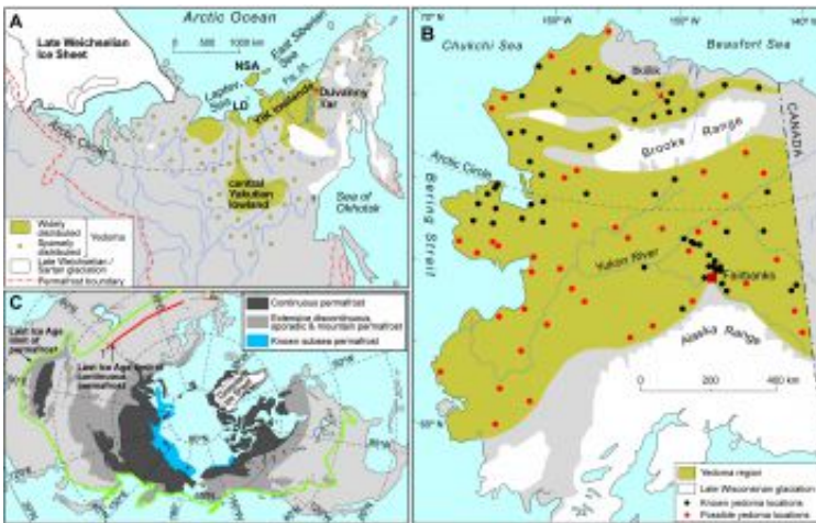
Maps showing yedoma distribution
