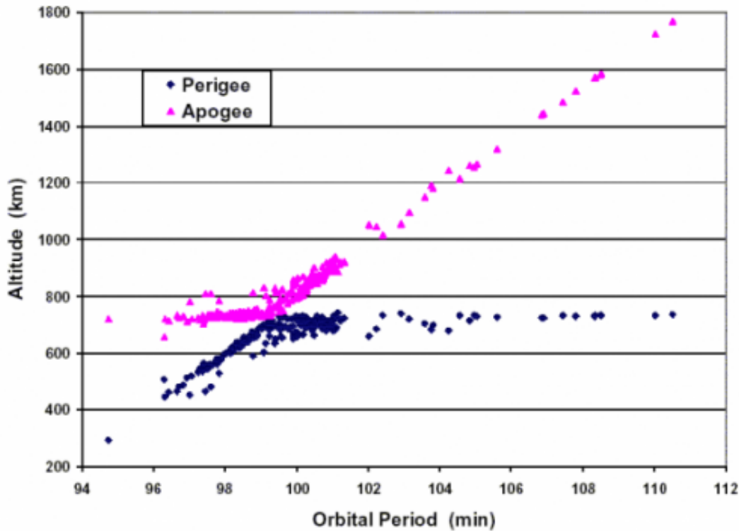
Gabbard diagram displaying a sample disintegration of a Long March 4 booster in 2000. Credit: the NASA Orbital Debris Office
