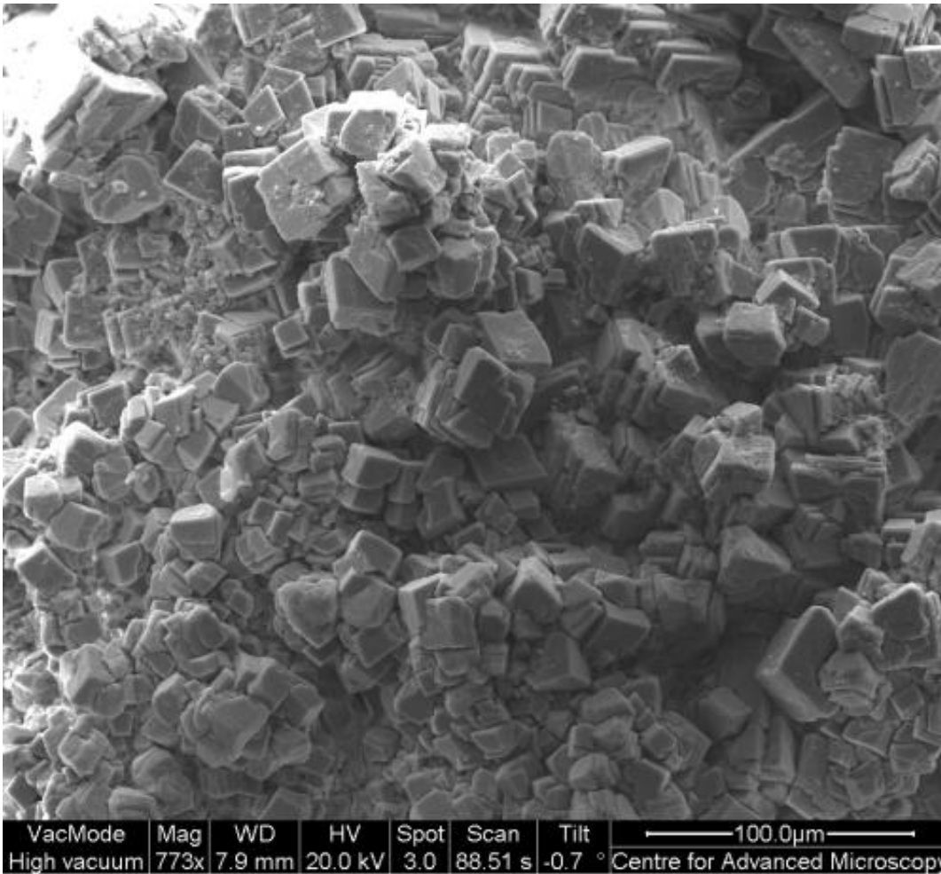
Image of a ball of calcium carbonate taken using an electron microscope (Reading Centre for Advanced Microscopy) Credit: Professor Mark Hodson
