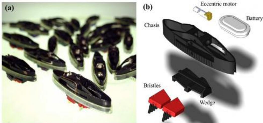
(a) A collection of the BBots used in the experiment. (b) Schematic of an individual BBot. A plastic chassis is connected to a pair of toothbrushes via a slanted wedge. An eccentric motor is positioned on the top side of the device and is powered by a VARTA rechargeable button-cell battery. Credit: L. Giomi et al, arXiv:1302.5952
