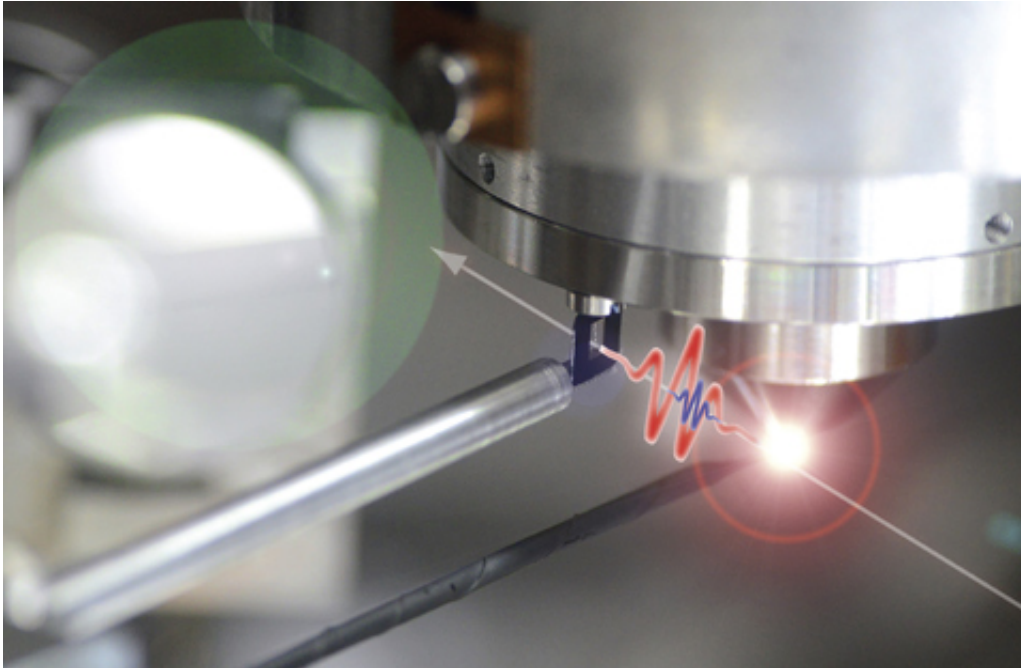
Figure 2: Attosecond real-time observation of changes in the electronic properties of a dielectric induced by the oscillating field of light. A nanometric thin silica-glass film (black frame in the centre of picture) is exposed to intense few-femto-second light pulses (red). The strong field of the light pulse changes the electronic states in the glass, with each cycle of its oscillation. These variations are tracked in real time by a series of "snapshots" recorded by attosecond light pulses (blue) passed through the sample at different instants delayed with respect to the intense excitation pulse. The recorded attosecond snaps of the instantaneous state of the electronic system of the probed sample; from these snaps the field-induced changes can be reconstructed in "slow-motion replay". Photo: Thorsten Naeser, LMU
