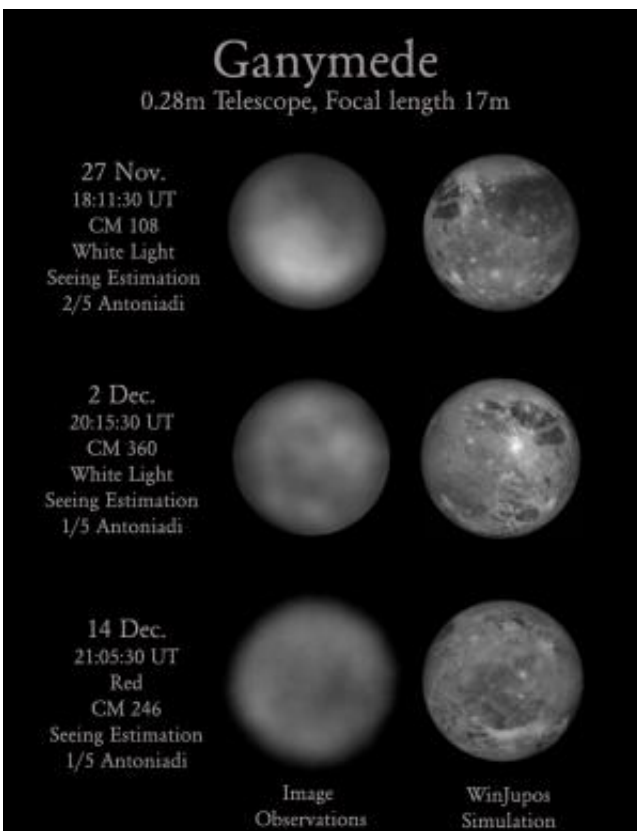
Albedo maps of Ganymede (left) and how they relate to known surface features (right). Credit: Manos Kardasis
