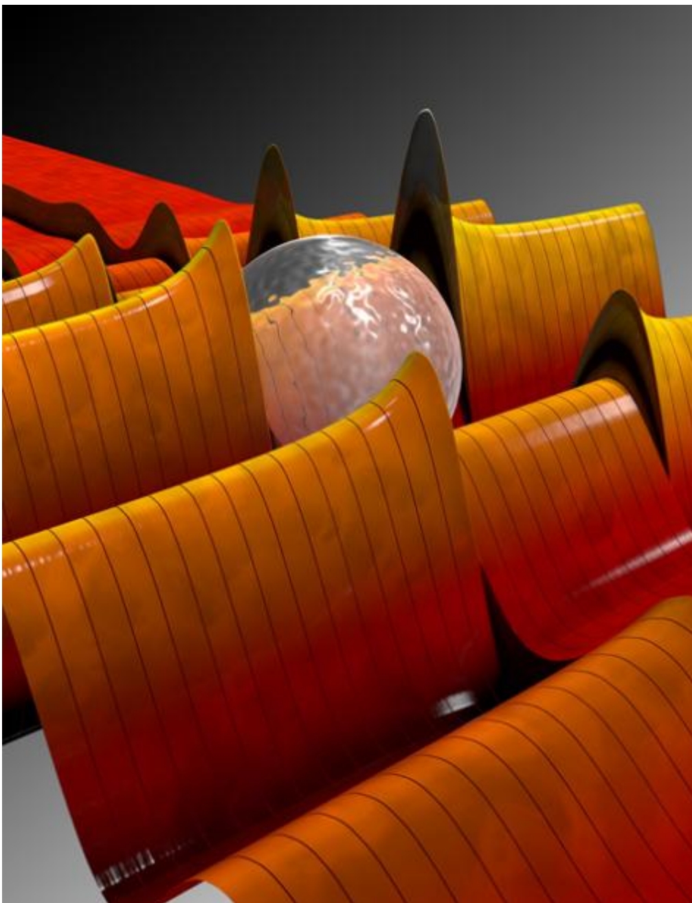
Figure 2: Amplified near-fields at the poles of a silica nanosphere. The local field on the polar axis is plotted as function of time, where time within the few-cycle wave runs from the lower right to the upper left. The fields show a pronounced asymmetry along the polarization axis of the laser (i.e. along the rims and valleys of the wave). This asymmetry leads to higher energies gained by electrons on one side of the nanoparticle as compared to the other side. For the given example the most energetic electrons are emitted from the backside, where the highest peak field is reached. The energies of the electrons and their
