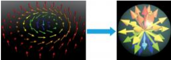
Figure 1: In a skyrmion (left) the electron spins, represented as arrows about which the electrons are rotating, are arranged such they map onto the surface of a sphere (right). Credit: 2011 X. Z. Yu et al.
