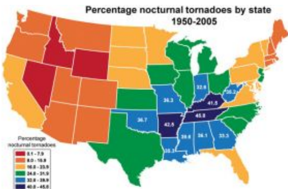
Percentage of nocturnal tornadoes by state
