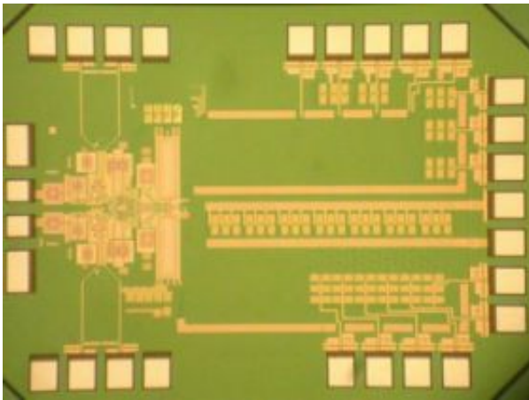
Microphotograph of IMEC's full CMOS multiple antenna receiver for 60GHz (1400 \mu m \times 1000 \mu m)
