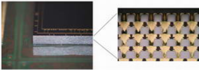
Cross section of test sample stacked multi-chip
